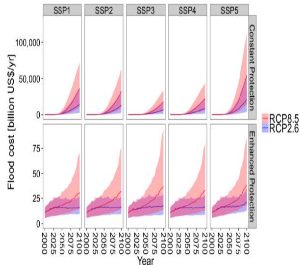
Fig. 55. Global expected annual flood cost. The lines show the average impacts across the range of DEMs, population datasets, GCMs, and land-ice scenarios used. The shaded areas show the respective uncertainty ranges defined by the maximum and minimum impacts.
