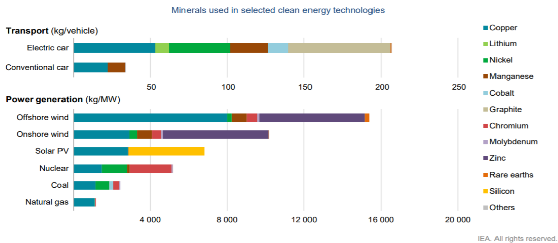
Figure 30. Comparative mineral intensities of conventional and “clean” technologies
