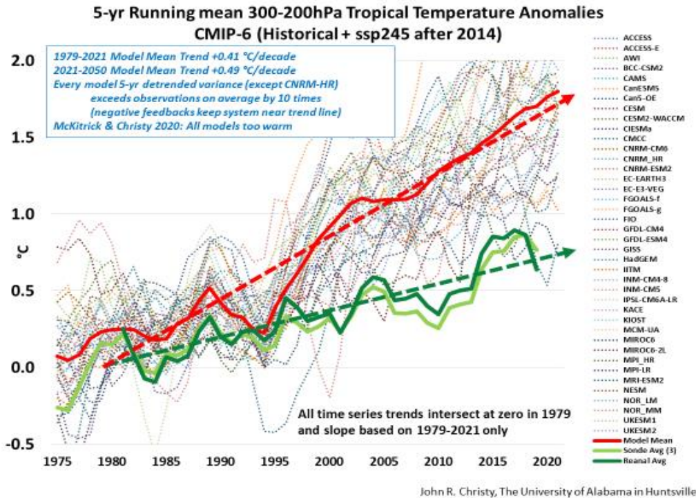
Figure 3. The CMIP6 model suite compared to observations.
