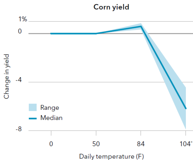
Figure 18. Corn Yield vs. Temperature
