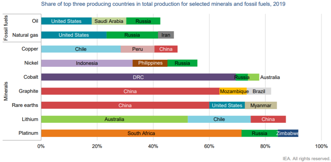
Figure 33. Top three producing countries, fossil fuels and ETMs
