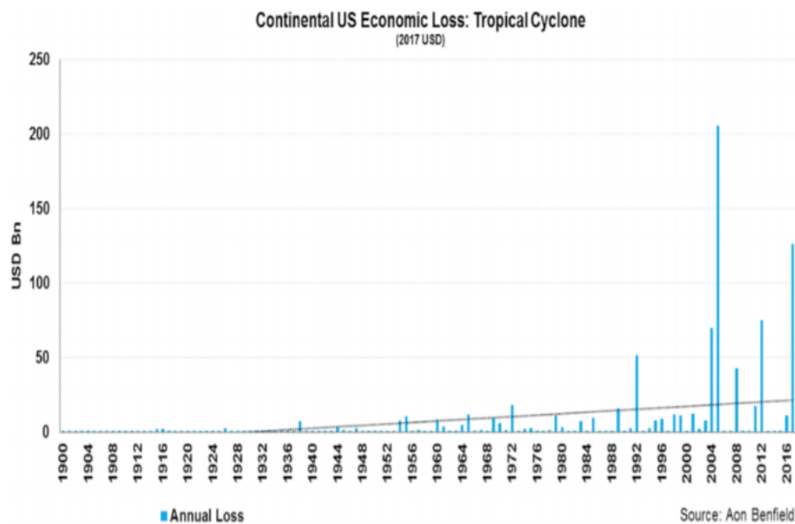
FIG. I. CONUS total inflation-adjusted economic losses from TC landfalls (1900–2017). The dotted line represents the linear trend over the period. The p value for the linear trend is <0.01 , indicating that the trend is significant.
