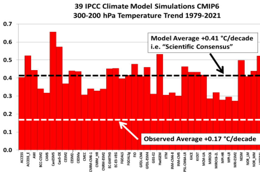
Figure 5. CMIP 6 models vs. observations. Source: John Christy.
