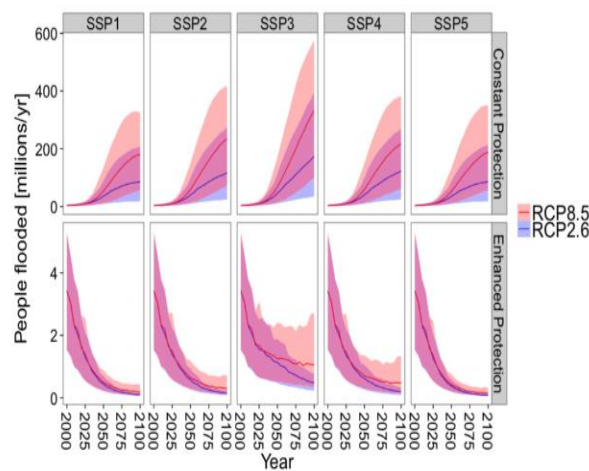
Fig. 54. Global expected annual number of people flooded. The lines show the average impacts across the range of DEMs, population datasets, GCMs, and land-ice scenarios used. The shaded areas show the respective uncertainty ranges defined by the maximum and minimum impacts.
