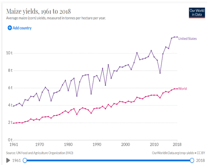
Figure 21. Corn Yields, US & Global
